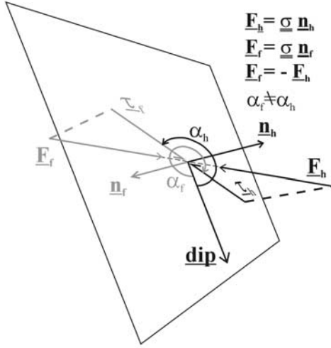
Figure 2. Forces ( (\underline{F}_f) and (\underline{F}_h) ) and their shear components ( \underline{\tau}_f and \underline{\tau}_h ) acting between the two sides of a fault surface element in a stress field represented by the stress tensor \underline{\sigma} . The shear direction ( \underline{\alpha} ) is defined by the angle between the dipline and the shear vector (equation (12)). See text for further discussion.
