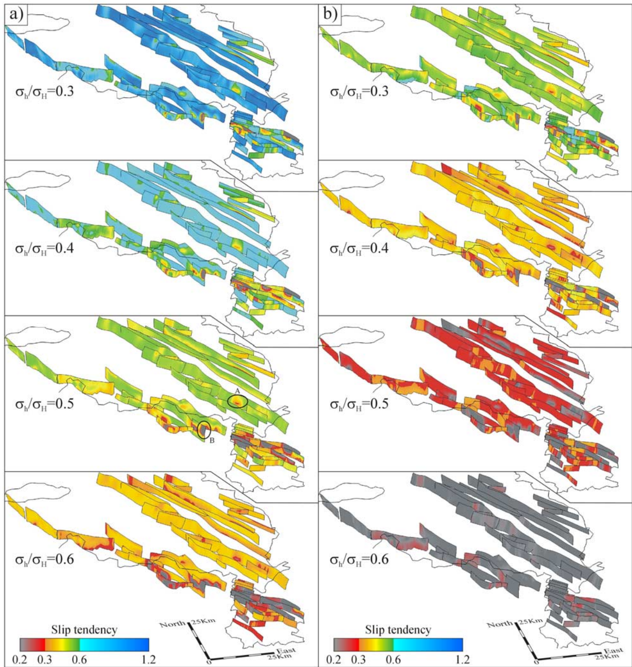
Figure 6. Perspective view of the 3-D faults with slip tendency patterns calculated for input stress tensors having different \sigma_h/\sigma_H ratios and \sigma_H directions of N145 degrees. Vertical scale is 4\times exaggerated. (a) Stress tensors describing a normal faulting regime. (b) Strike-slip-faulting stress tensors. The R-value of the stress tensor was modelled as 0.45 for Figure 6a and as 0.25 for Figure 6b representing the maximum slip tendencies within the modelled R-value range.
